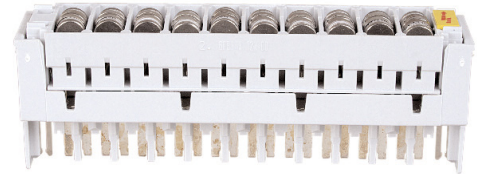
Protection Magazine 10 pair
